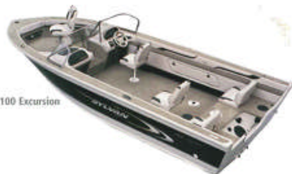
2100 and 1900 Excursion Bow Livewell/Backwell
